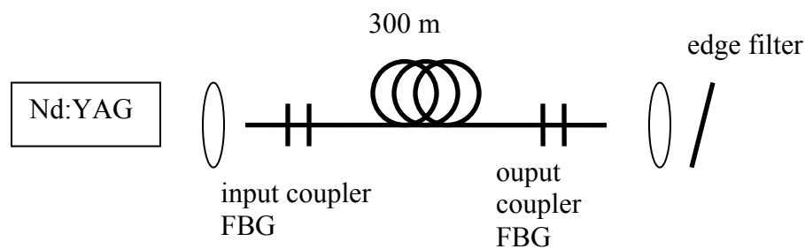
Figure 58. Experimental setup of an RFL based on a multimode graded-index fiber.
