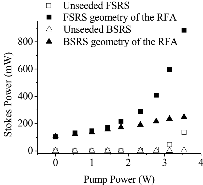
Figure 33. Stokes power as a function of coupled pump power for the FRSR geometry (squares) and the BSRS geometry (triangles). The output of unseeded SRS (unfilled figures) and the RFA (filled figures) are shown.
