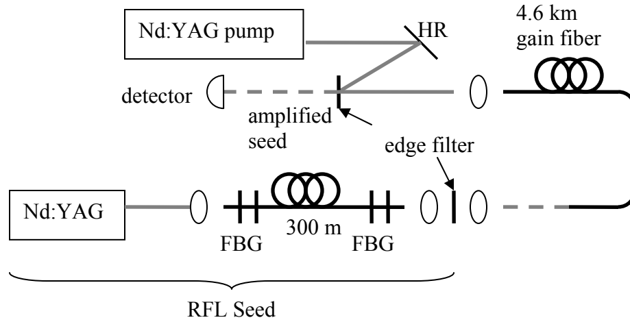
Figure 15. Experimental setup for characterizing the performance of the BSRS geometry of an RFA based on a graded-index fiber. An RFL provided the seed.
